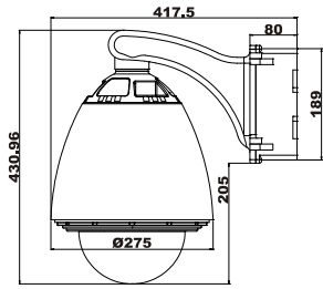
External Dimensions
